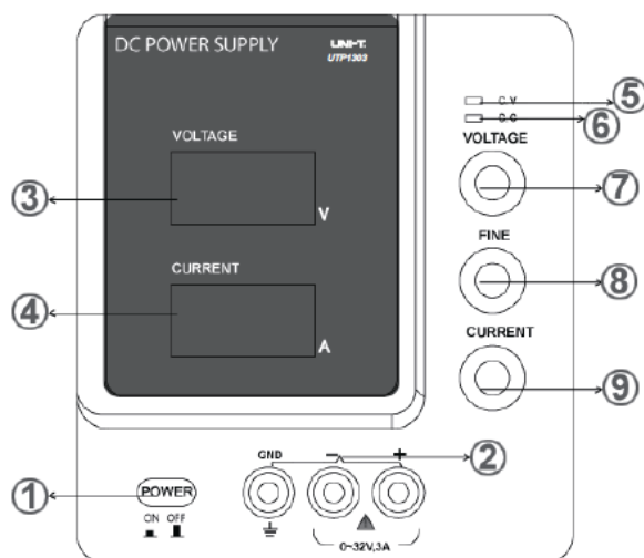
Figura 2 – Panoul frontal: Modelele UTP1303 / UTP1305
